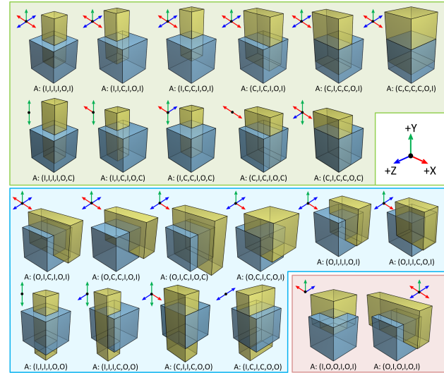
Figure 8: The 23 cases of ICO vector ( A ), in which 3D boxes A (yellow) and B (blue) intersect; ordered by +x , -z , -x , +z , +y , and -y . The arrows show the possible axial movement directions of A over all joint geometries that we may choose to use.
