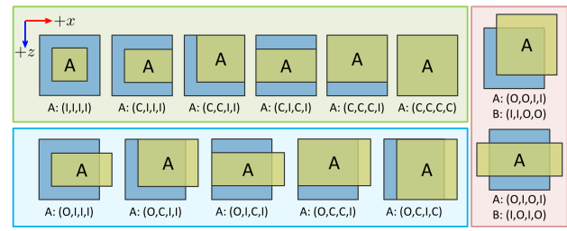
Figure 7: The 13 cases of ICO vector ( A ), in which 2D boxes A (yellow) and B (blue) intersect; ordered by +x , -z , -x , and +z .
