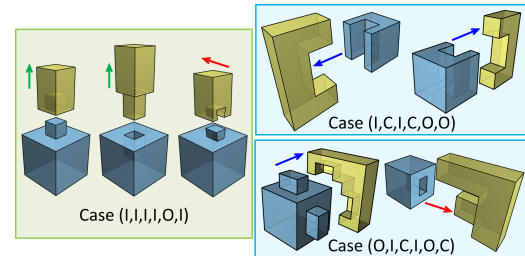
Figure 9: Example joint geometries for some cases in Figure 8.
