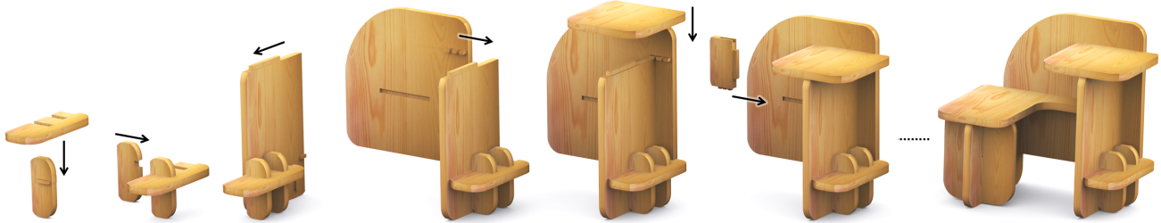
Figure 1: Some snapshots showing the assembly of MULTI-FUNCTION TABLE. Our method can plan a network of joints (e.g., Figure 2) that globally interlocks the component parts in the assembly; the input component parts are just simple 3D shapes without joint geometry.
